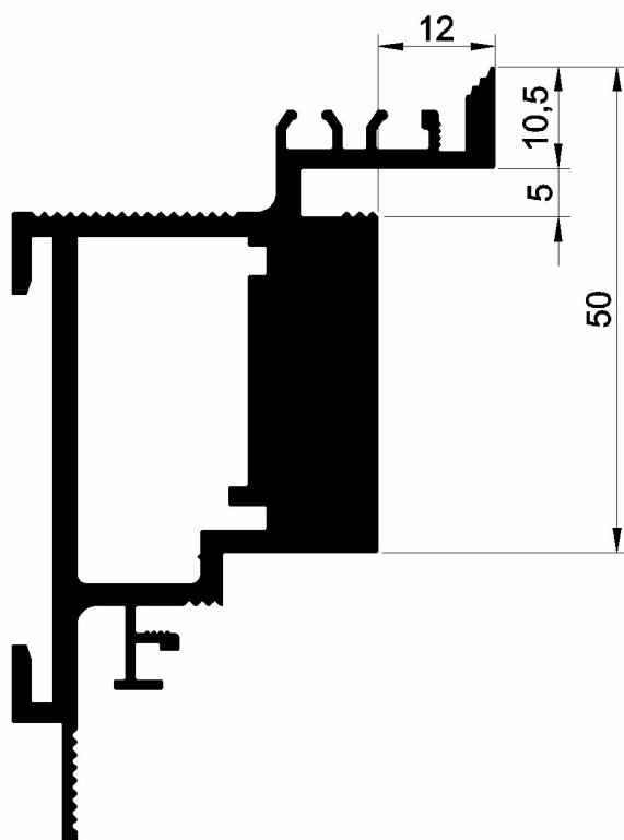
rebate dimension for 5mm door seal
