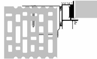
Mod. TCT
